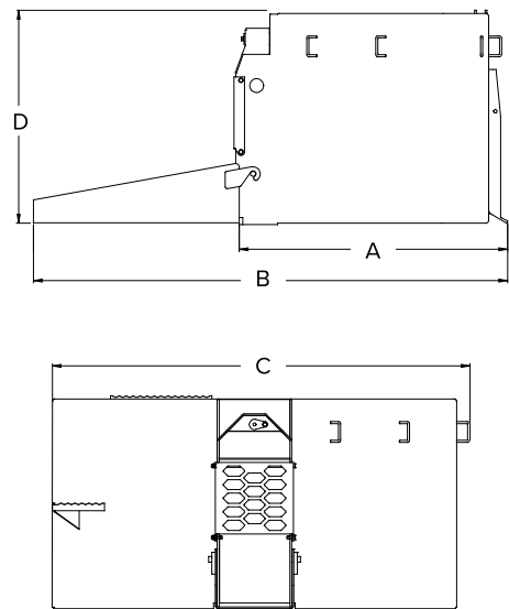
3/4 yard Concrete Chuter
