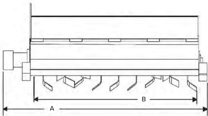
TILLER (FITS COMMON INDUSTRY INTERFACE MOUNT)
